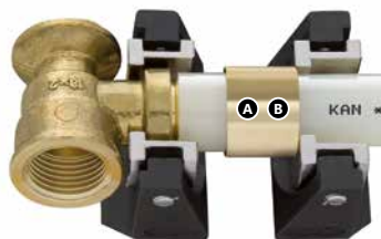
Installation of brass wallplate elbows
