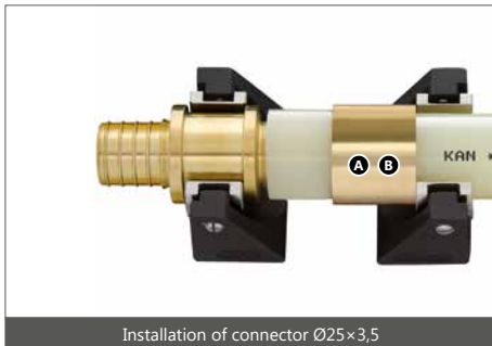
Installation of connector \text{Ø}25 \times 3,5
